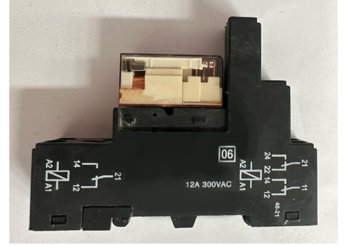
6. 24V relay $ 19.60
