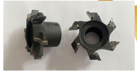
15 Milling knife $ 42.60
